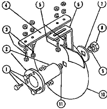
FIG. 6 — FURROW FILLER ATTACHMENT MACH. NO. 200080
