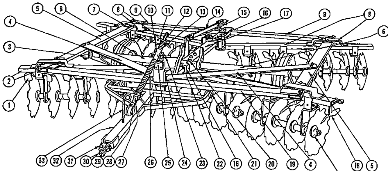
FIG. 1 — MODEL 200101 WHEEL MOUNTED TANDEM HARROW
