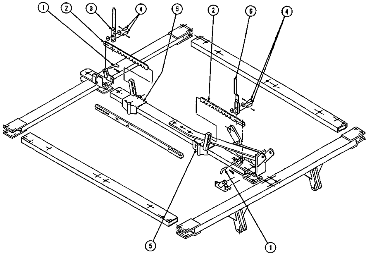
FIG. 3 — CENTER FRAME ASSEMBLY WITH RATCHET TYPE, DISC GANG ANGLING CHANGE
