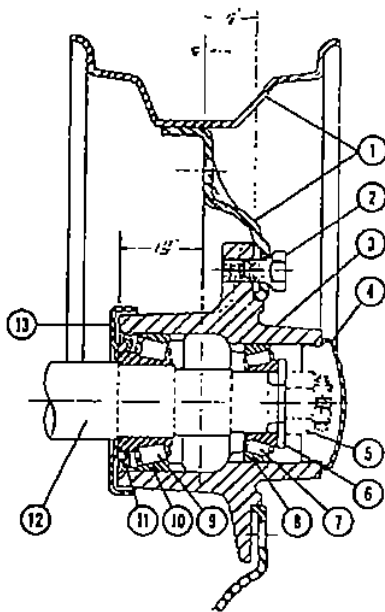
FIG. 5 — WHEEL HUB ASSEMBLY SEE ITEM 17
