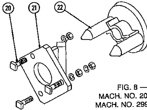
FIG. 6 — FURROW FILLER ATTACHMENT MACH. NO. 200080
