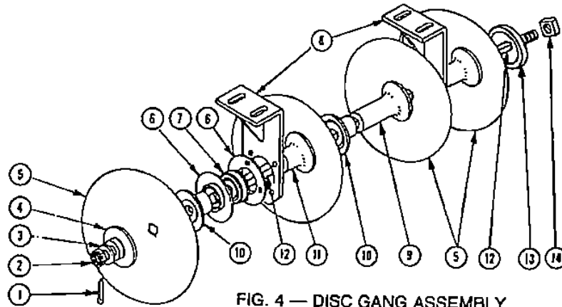
FIG. 4 — DISC GANG ASSEMBLY
