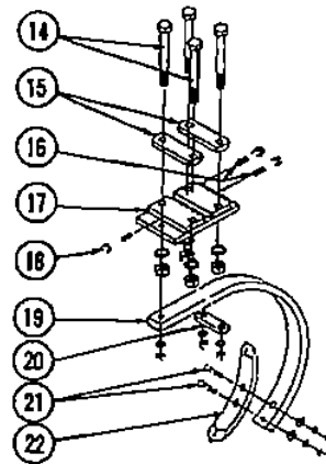
BALK BREAKER ATTACHMENT MACH. NO. 299054 REPAIRS ONLY
