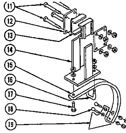
FIG. 7 — BALK BREAKER ATTACHMENT MACH. NO. 299089
