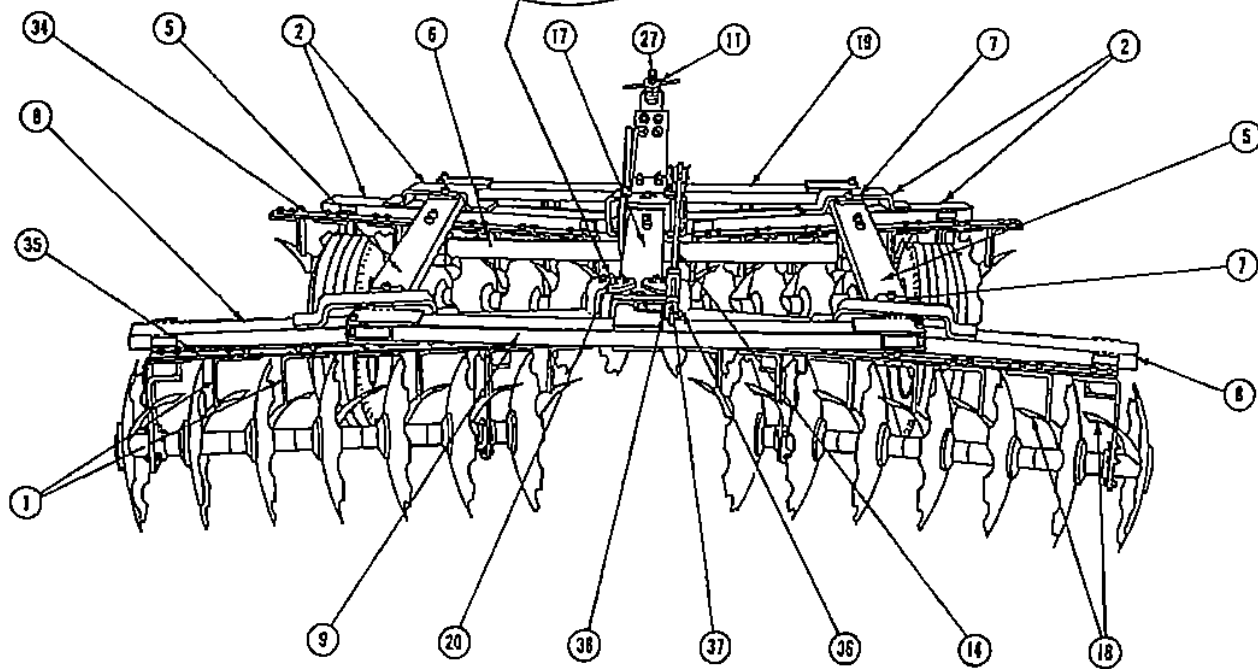
FIG. 2 — MODEL 200113 WHEEL MOUNTED TANDEM HARROW
