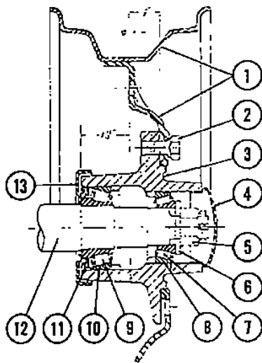
WHEEL HUB COMPLETE — SEE ITEM 14. REPAIR KIT — SEE ITEM 15.
