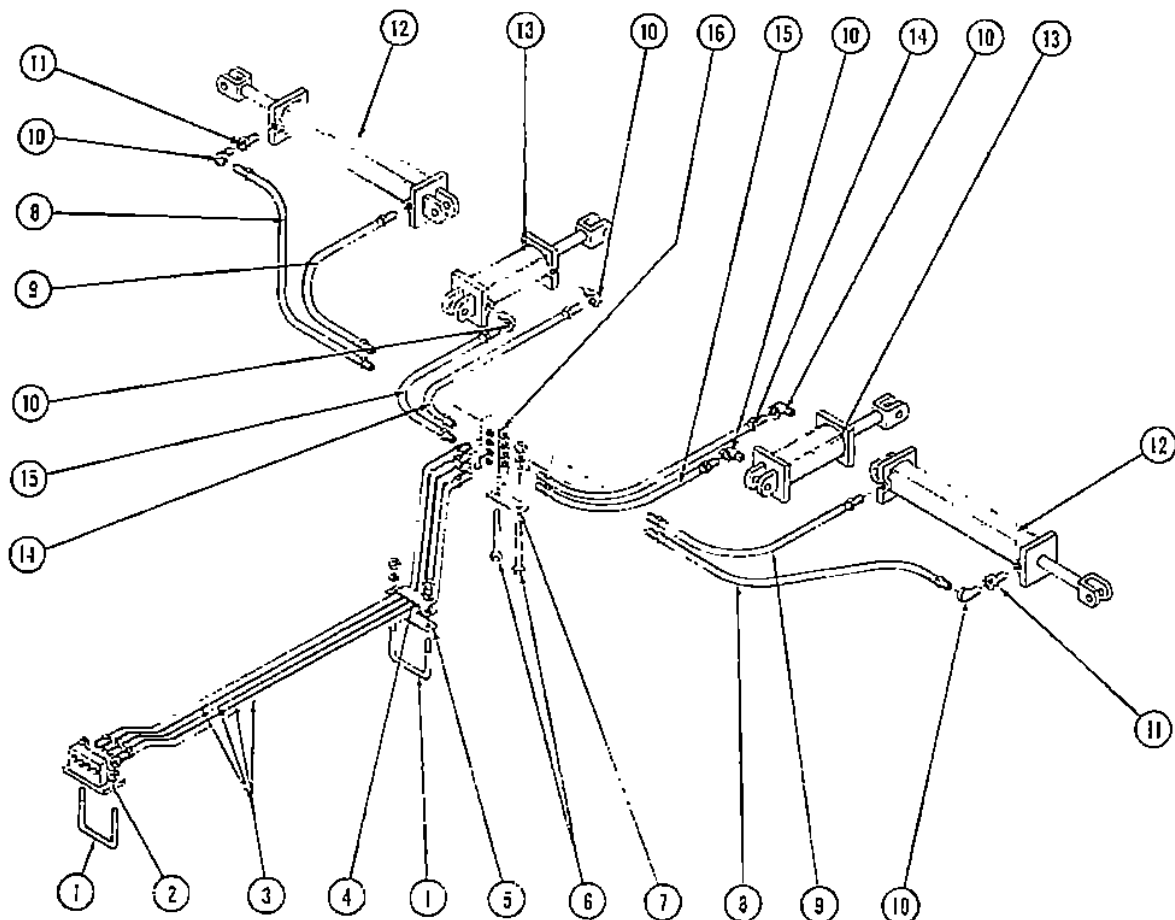
FIG. 6 — HYDRAULIC ASSEMBLY
